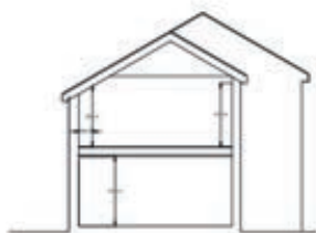
Shedding System Section Scale 1/8" = 1'-0"
