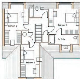
First Floor Plan Scale 1:100
