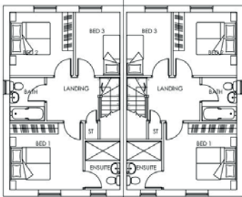
FIRST FLOOR PLAN 1:50
